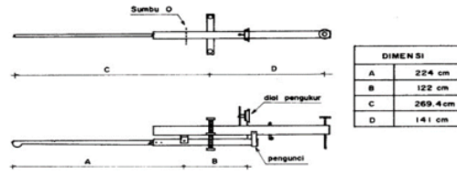
Gambar 2 Alat Benkelman Beam
