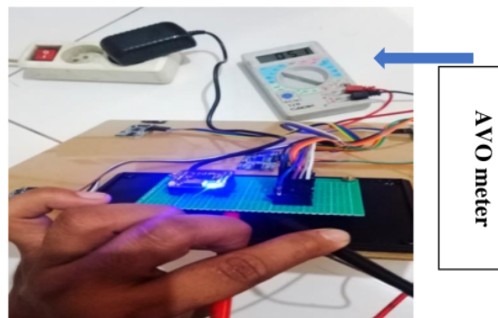
Gambar 12. Pengujian adaptor power supply
