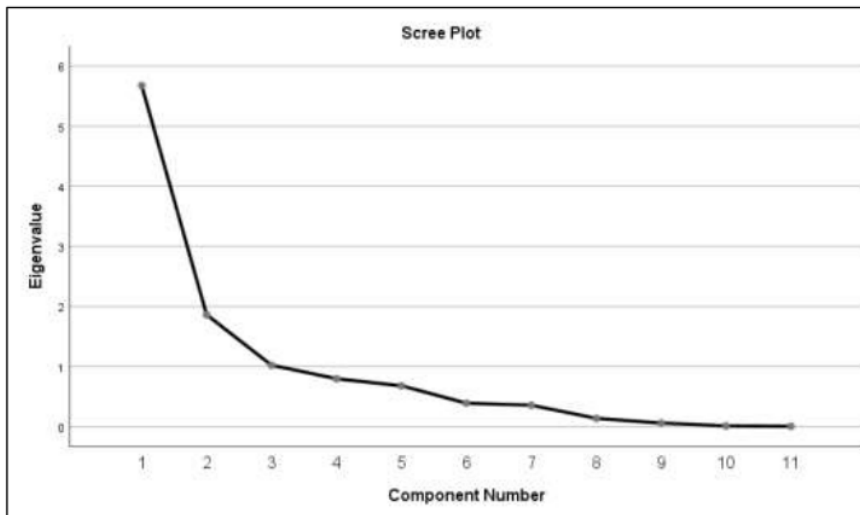
Gambar 3. Scree Plot
