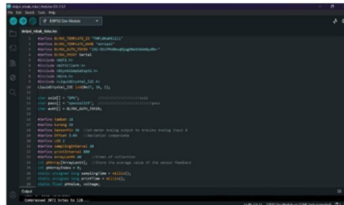
Gambar 2. Software ESP 32
