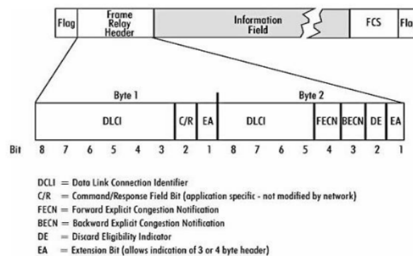
Gambar 2. Metode Frame Relay
