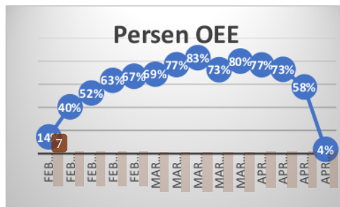
Gambar 5 Hasil Perhitungan OEE
