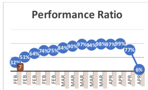
6 Gambar 3 Hasil Perhitungan Performance Ratio
