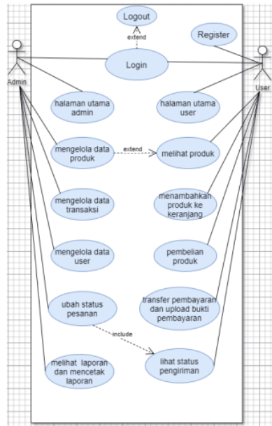
Gambar 1. Use Case Diagram
