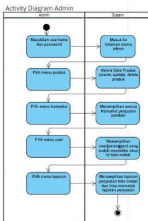
Gambar 4. Activity Diagram Admin
