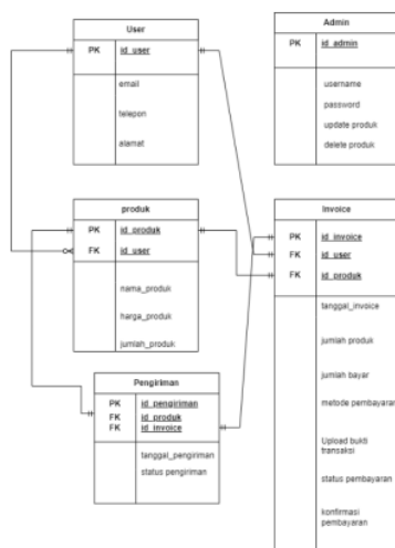
Gambar 5. Tabel Entity Relationship Diagram
