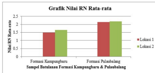
Gambar 4 Grafik hasil rata-rata rebound number
