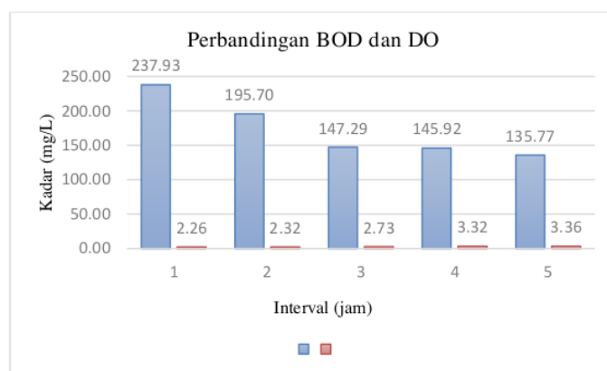
Gambar 4. Diagram Perbandingan Kadar BOD dan DO
