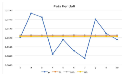
Peta Kendali ( Control Chart )
