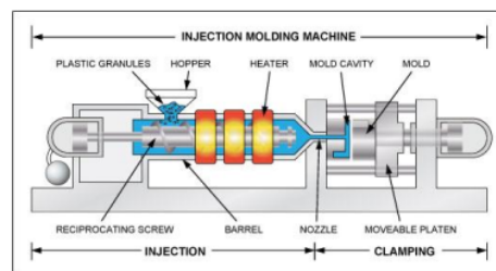
Gambar 2.. Proses Injection Molding
