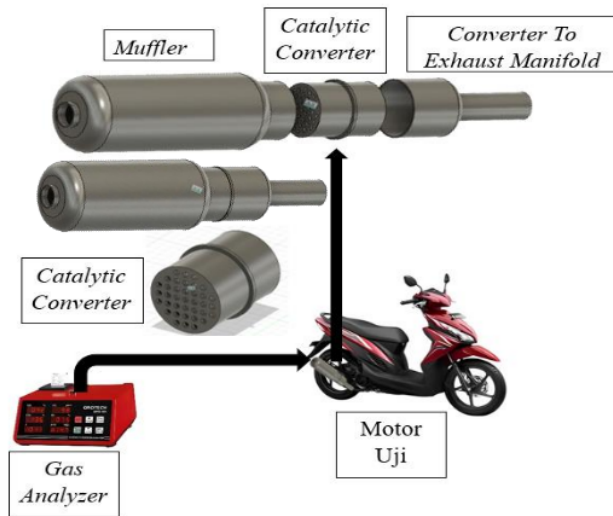
Gambar 3.1 Setting Peralatan Penelitian
