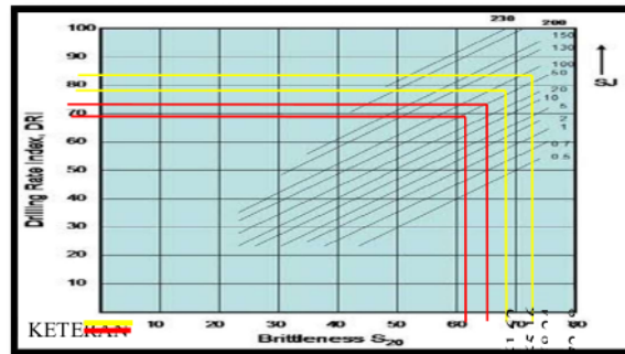
Gambar 2 Grafik Nilai Drilling Rate Index (DRI)
