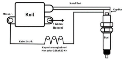
Gambar 1. Rangkaian Plasma Capacitor Igniton
