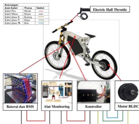
Gambar 3.1 Setting Alat Penelitian
